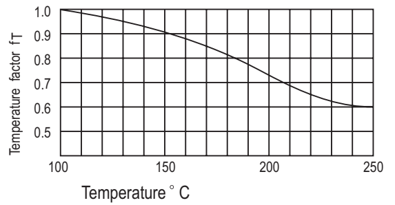
Fig. 9 Temperature factor
